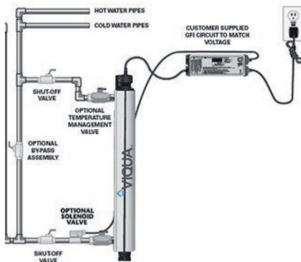
Installationskiss
