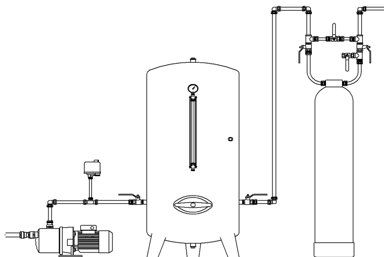
Installationskiss
