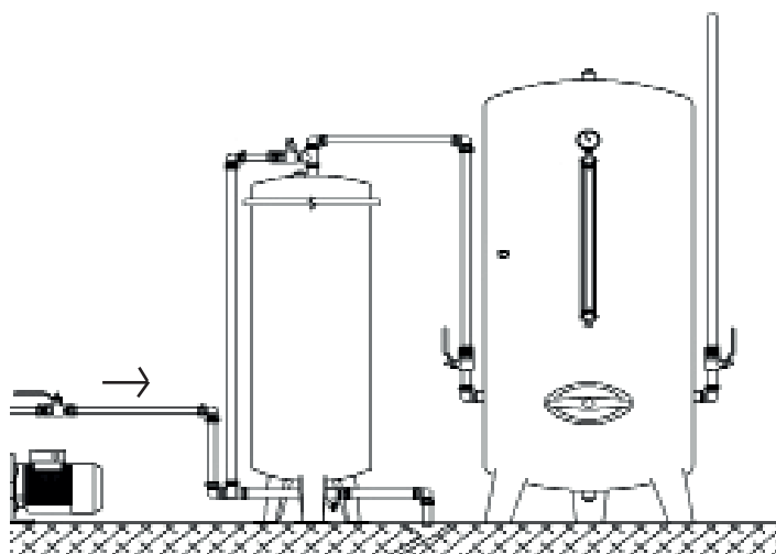
Installationskiss
