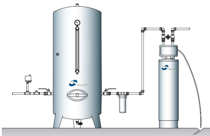
Installationskiss
