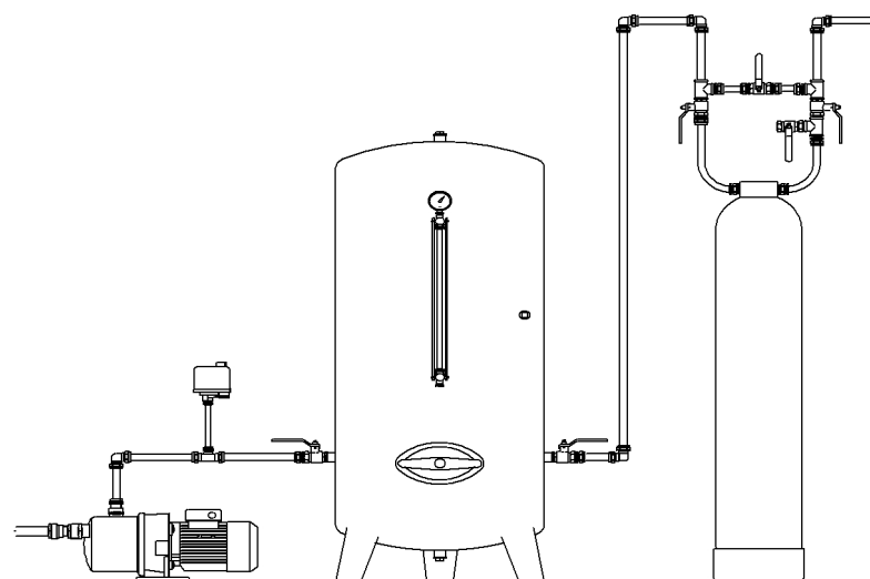
Installationskiss
