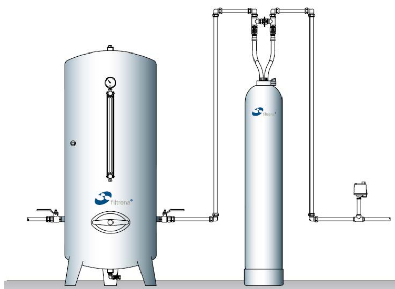
Installationskiss
